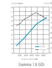
Gamma 1.6 GDI
