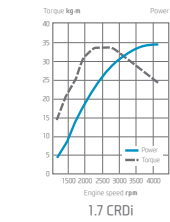
1.7 CRDi
